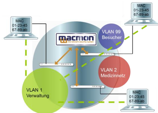
Abb. 1: macmon VLAN-Management
